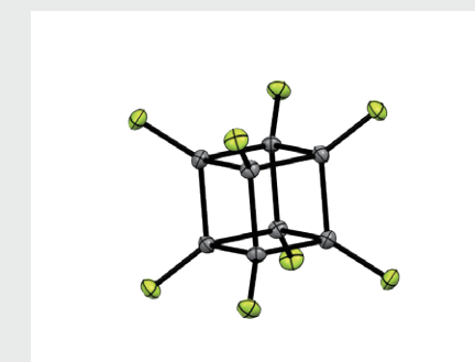
Perfluorocubane (White: Carbon, Yellow: Fluorine)
