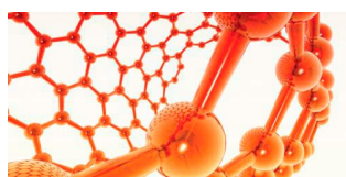
Materials (Nanotechnology)
